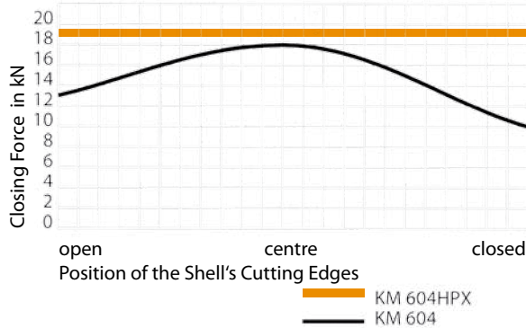
Comparison of Closing Forces
