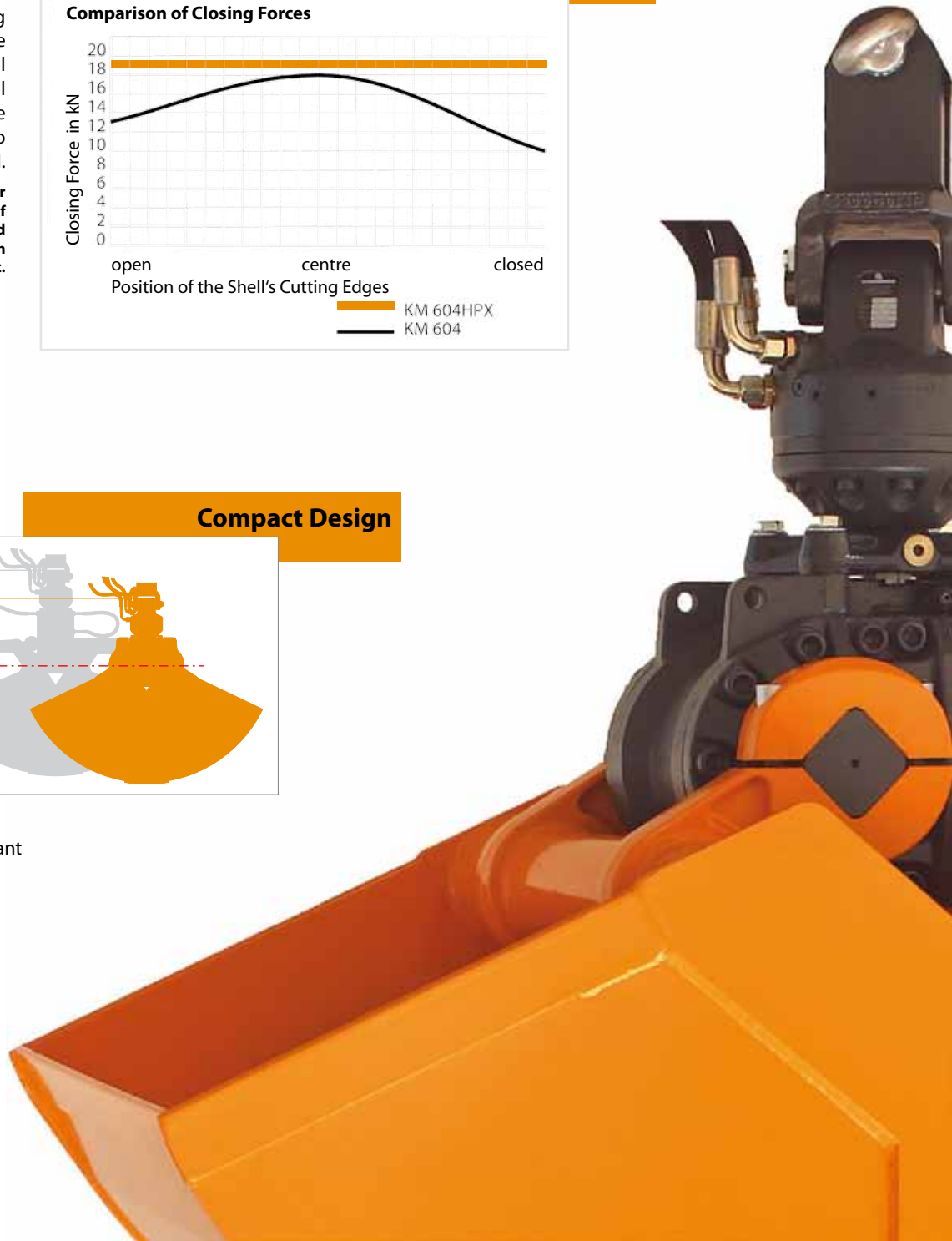
Comparison of Closing Forces
